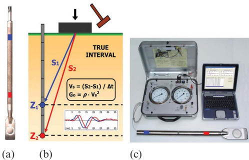
Figure 1. Seismic dilatometer test (Marchetti et al. 2008): DMT blade and seismic module (a); schematic test layout (b); seismic dilatometer equipment (c).
