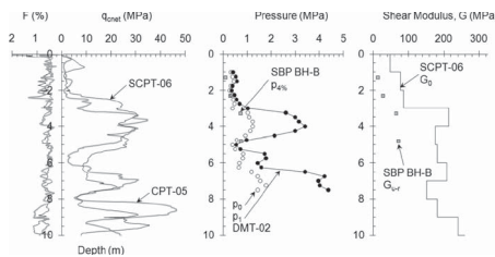
Figure 8. CPT, DMT, SBP and SCPT parameters at Ledge Point: Friction ratio F , tip resistance q_{cnet} , pressure and shear modulus G_0 profiles, (Schneider & Lehane 2010).
