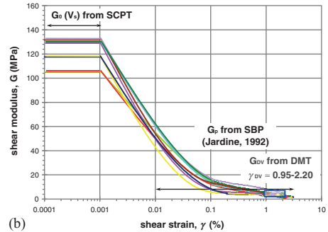
Figure 5. G - \gamma decay curves from SBP and SCPT tests and G_{DMT} ; (a) and G_{DV} ; (b) Values from DMT tests.
