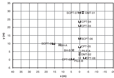
Figure 7. Ledge Point test site (Schneider & Lehane 2010).
