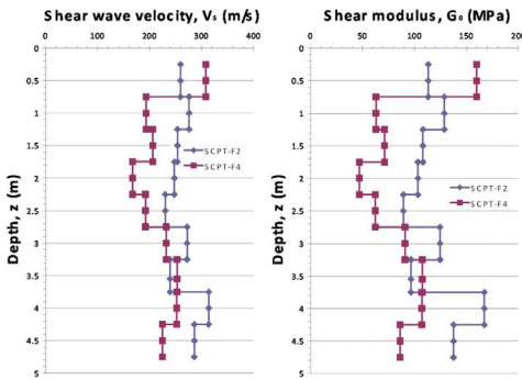
Figure 4. SCPT results at Shenton Park: Shear wave velocity V_s , shear modulus G_s .
