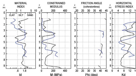
Figure 9. DMT results at Ledge Point: Material index I_D , constrained modulus M_{DMT} , friction angle \phi' , horizontal stress index K_D .
