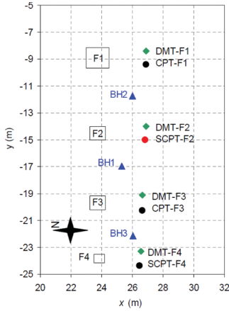
Figure 2. Shenton Park test site in 2006–2007 (Schneider et al. 2008).
