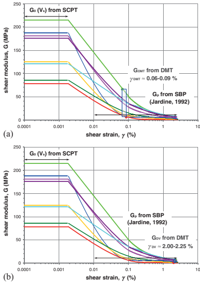
Figure 10. G_s - \gamma decay curves from SBP and SCPT tests and G_{DMT} (a) and G_{DV} (b) values from DMT tests.
