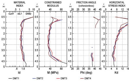
Figure 3. DMT results at Shenton Park: Material index I_D , constrained modulus M_{DMT} , friction angle \phi , horizontal stress index K_D .
