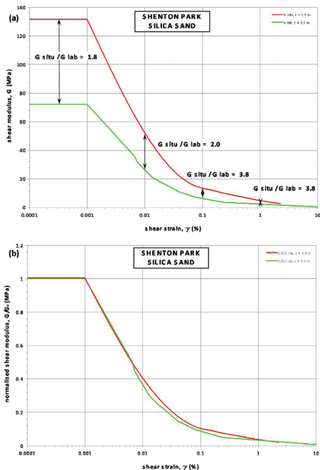
Figure 6. Shenton Park: Comparison (depth 3.9 m) between in situ and laboratory G - \gamma decay curve (a) and between normalized in situ and laboratory G/G_{0,\gamma} decay curve (b).
