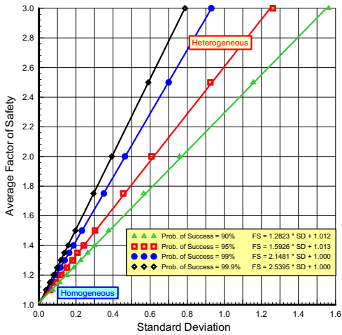
Figure 3: Design Chart of Beta Probability Distribution Analyses for Slope Stability with Min/Max Limits = Average ± 3 Standard Deviations
