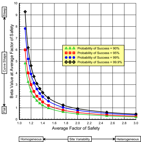
Figure 2: Beta Probability Analyses For Slope Stability with Min/Max Limits = Average ± 3 Standard Deviations
