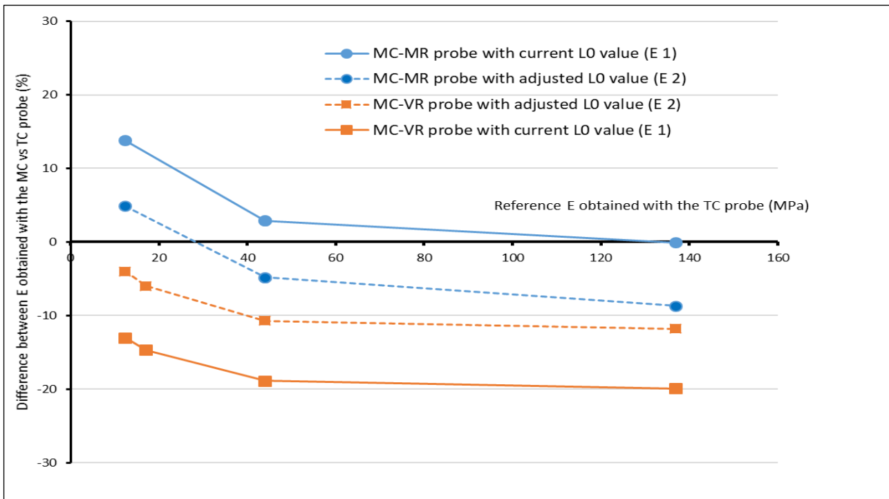
Figure 7. Difference in % between E obtained with MC vs TC probes before (E 1) and after (E 2) adjustment of L0
