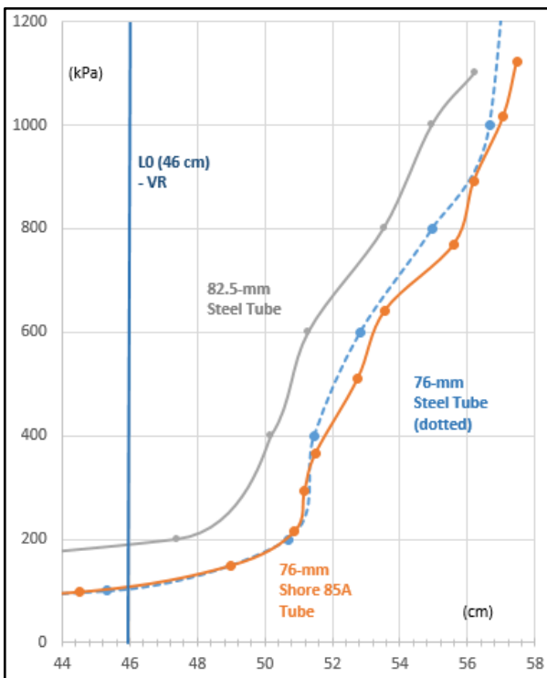
Figure 8. CL vs the stiffness and inner diameter of the TST
