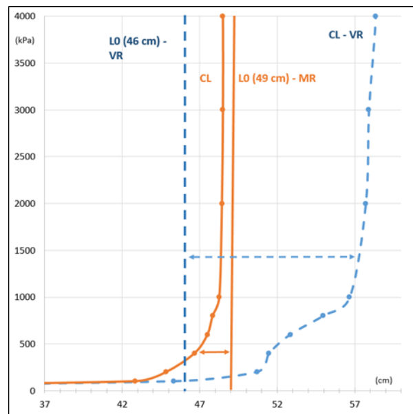
Figure 6. Evolution of CL versus L0 for MC - VR / MR probes
