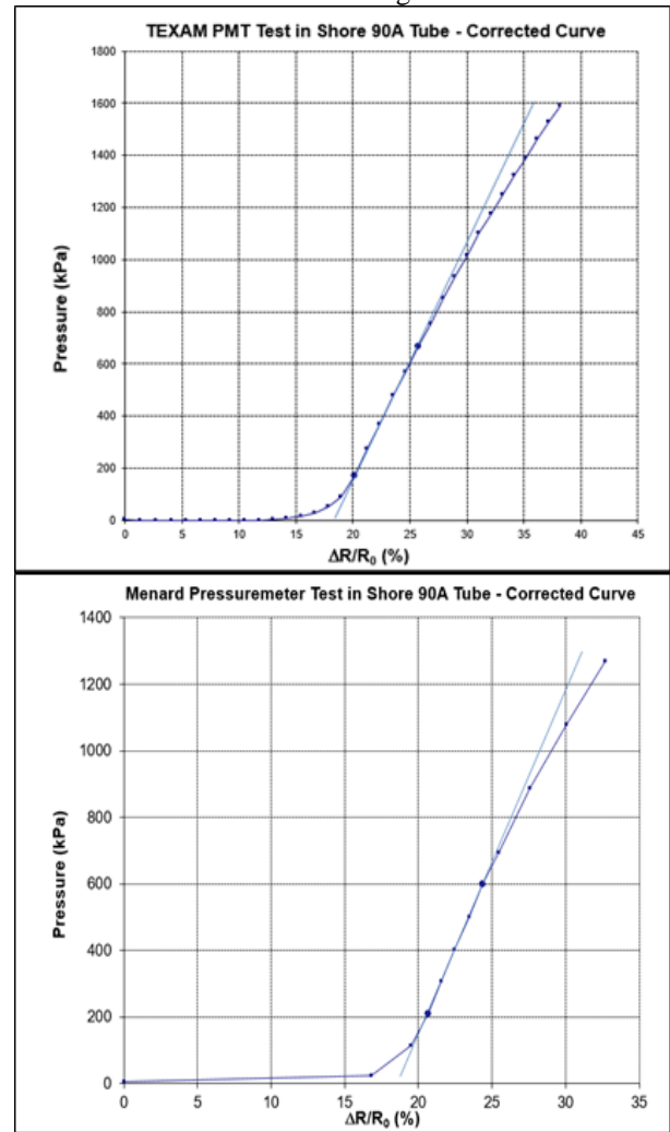
Figure 4. Typical test results in the Shore 90A TST obtained with N-size MC and TC Menard-type pressuremeters
