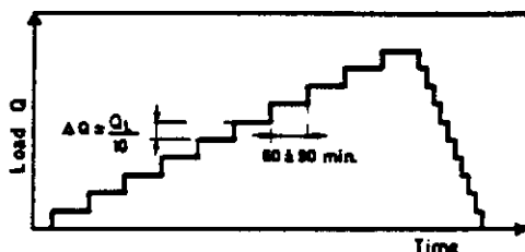
Fig. 1a). Schematic representation of loading programme according to LPC procedure.
