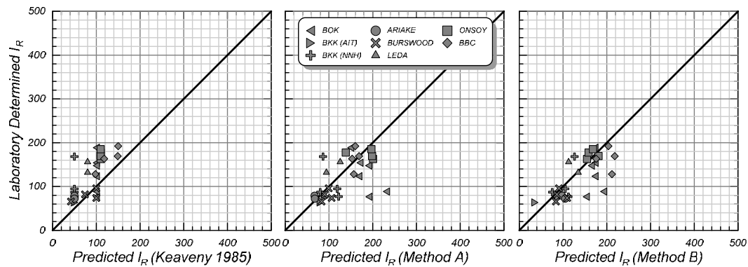
Figure 5. Comparison of predicted to measured rigidity index values using (left to right): Keaveny (1985), Empirical G_{50}/G_{max} based Method A, and Empirical G_{50} / G_{max} based Method B.
